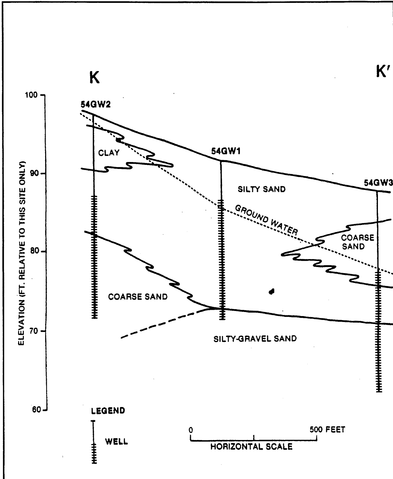
FIGURE 5-3* GEOLOGIC CROSS SECTION SITE 54: CRASH CREW BURN PIT CAMP LEJEUNE MILITARY RESERVATION SOURCE: ES&E, 1990 *54MW1 no longer exists.
