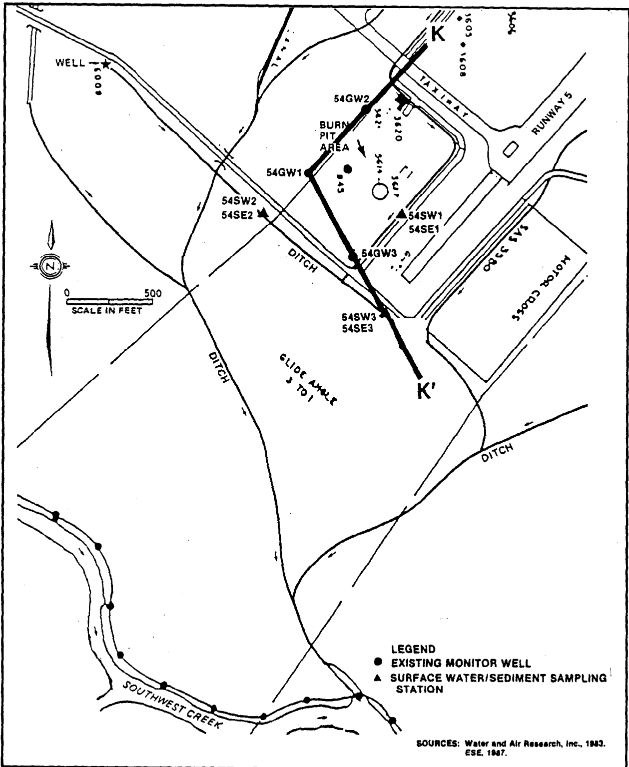
FIGURE 5-2* GEOLOGIC CROSS SECTION LOCATION SITE 54: CRASH CREW BURN PIT CAMP LEJEUNE MILITARY RESERVATION SOURCE: ES&E, 1990 *54MW1 no longer exists.
