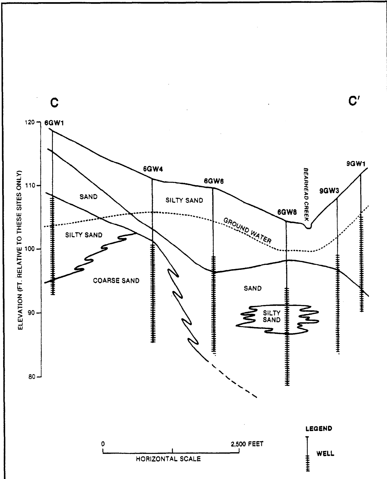
FIGURE 6-3 GEOLOGIC CROSS SECTIONS, SITES 6 AND 9, STORAGE LOTS 201 AND 203 AND FIRE FIGHTING TRAINING PIT SITE 82: PINEY GREEN ROAD VOC AREA CAMP LEJEUNE MILITARY RESERVATION SOURCE: ES&E, 1990
